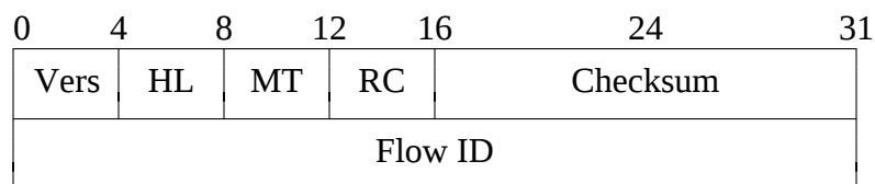
Fig. A.1. Encapsulation Protocol Header Example
